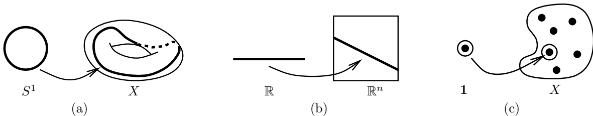
Figure 2: Mapping out of a basic object ( S^1 , \mathbb{R} , or \mathbf{1} ) picks out figures of the appropriate type (loops, lines, or elements).
